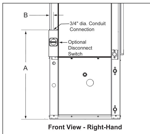
Figure 15: Optional disconnect switch location dimensions
