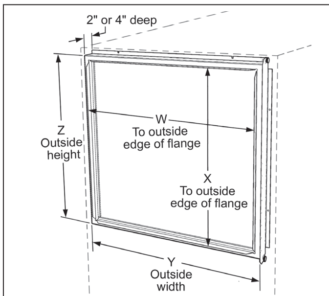
Figure 16: Optional filter rack dimensions - left-hand
