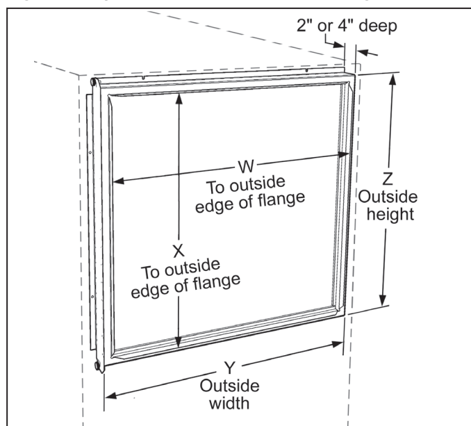
Figure 14: Optional filter rack dimensions - right-hand
