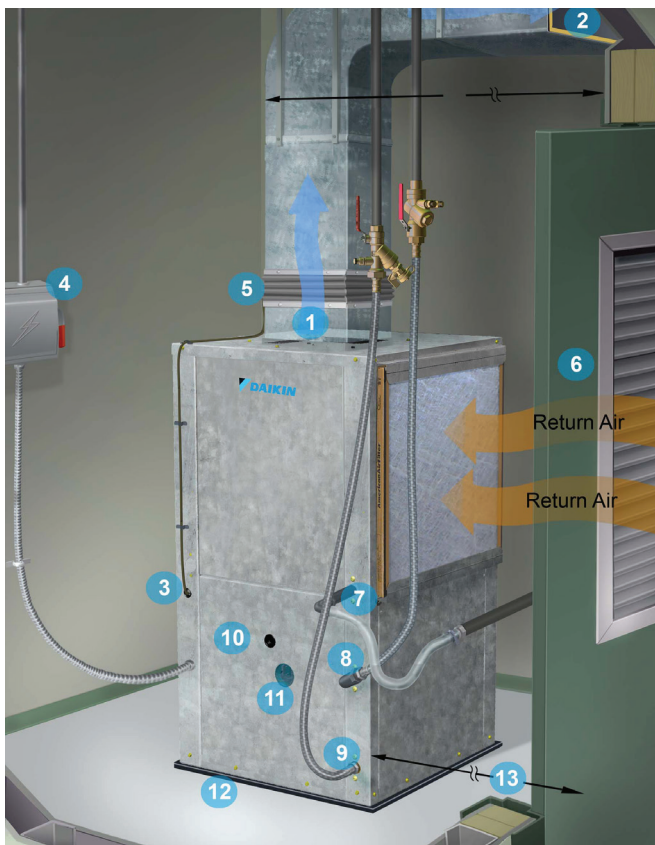
Figure 5: Typical closet installation - non-ducted application
