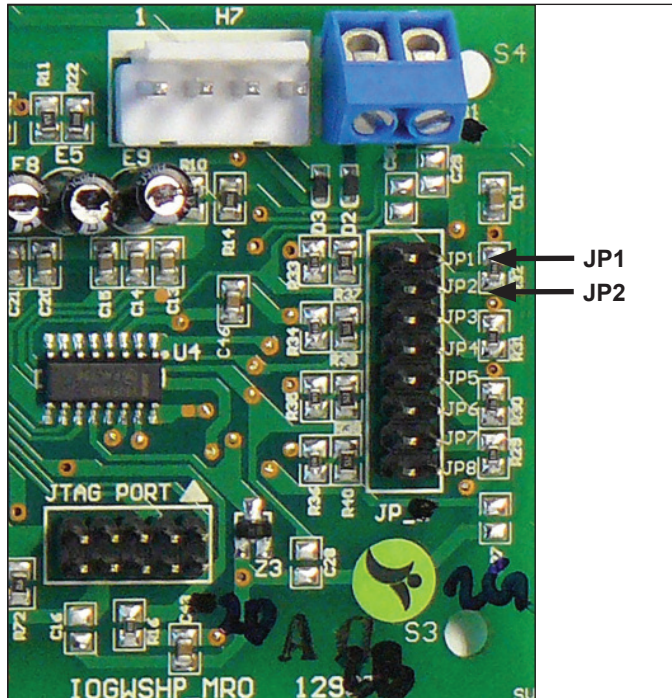
Figure 13: JP1 &amp; JP2 location on the I/O expansion module
