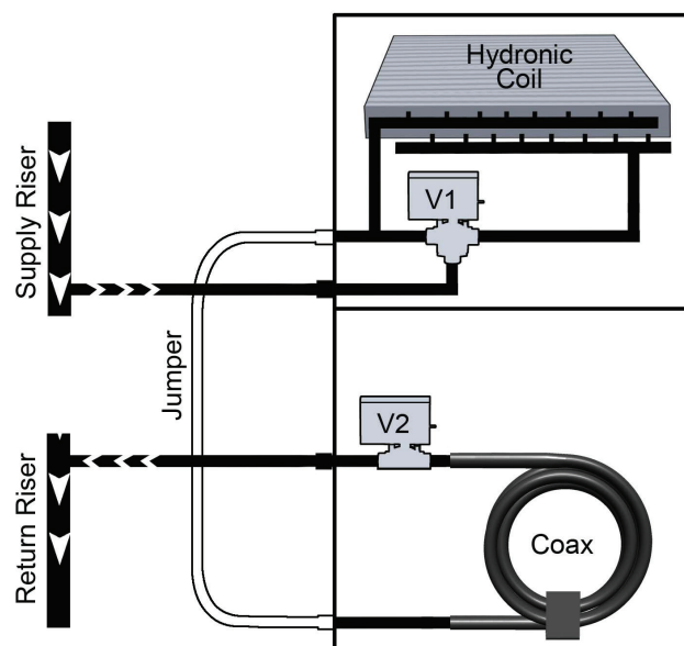
Figure 9: Piping schematic
